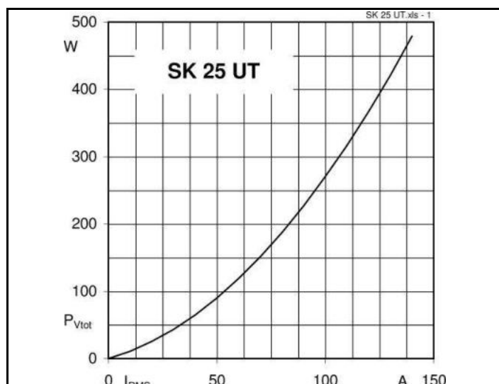
Fig. 1 Power dissipation per phase vs. r.m.s. current
